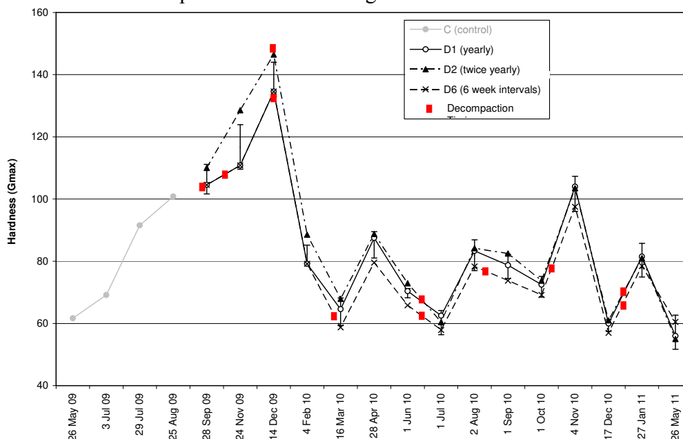
Figure 18. Surface hardness ( G_{max} of 70-80 is ideal, \geq 120 is concerning) of turf treatments (Control, D1, D2 and D6) from Phase 1 of the RTA trial. G_{max} values shown are of the 4 th drop from a 457 mm height.
