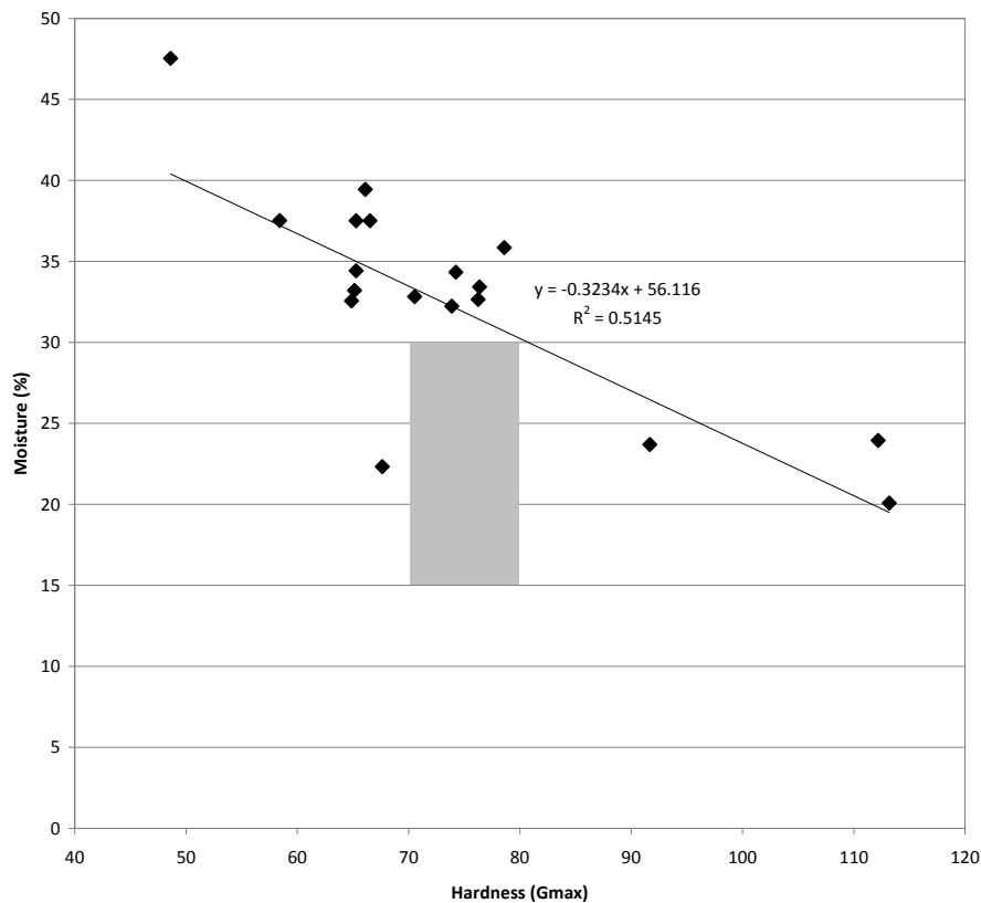
Figure 23. Correlation between soil moisture (%) and surface hardness (4 th drop G_{max} ) from the mean data collected within the C, D1, D2 and D6 subplots of fields 5 and 6 between 17 Mar 2010 and 23 Mar 2012. The recommended range (Henderson et al. , 2007) is highlighted in grey.
