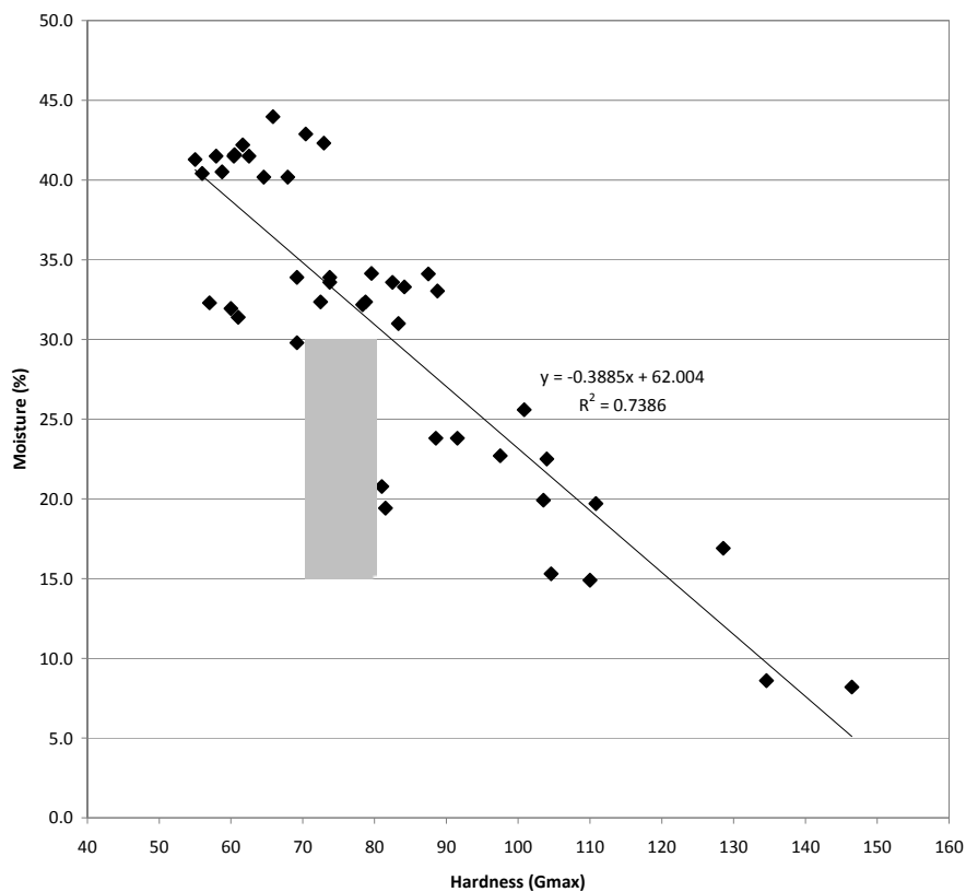
Figure 19. Correlation between soil moisture and surface hardness from the mean data collected within the Control, D1, D2 and D6 subplots of fields 3 and 4 between 9 Jan 2009 and 26 May 2011. The recommended range (Henderson et al. , 2007) is highlighted in grey.
