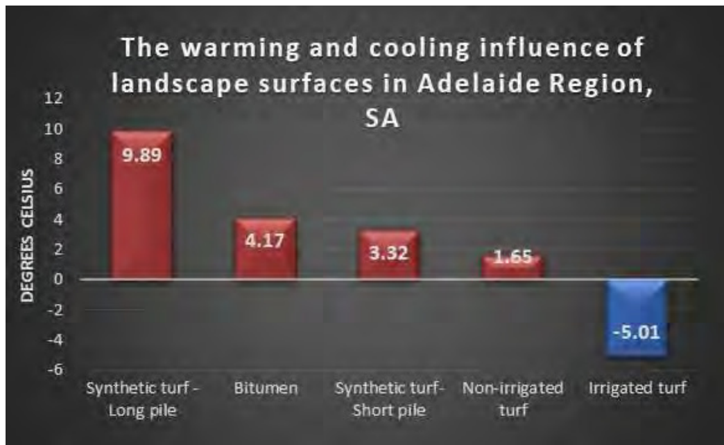
Figure 4). The thermal performance of non-irrigated living turf depends heavily on the seasonal precipitation during the year of data collection. During wetter years, non-irrigated living turf performs similarly to irrigated living turf (as illustrated by the Victorian data), while during drier years it performs more similarly to bitumen and other hard, dry surfaces (as illustrated by the South Australian data).
