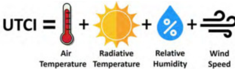
Figure 14. Conceptual equation of the Universal Thermal Climate Index (UTCI).
