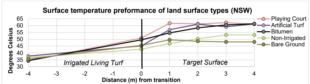
Figure 20. Surface temperature results of NSW thermal assessment.
