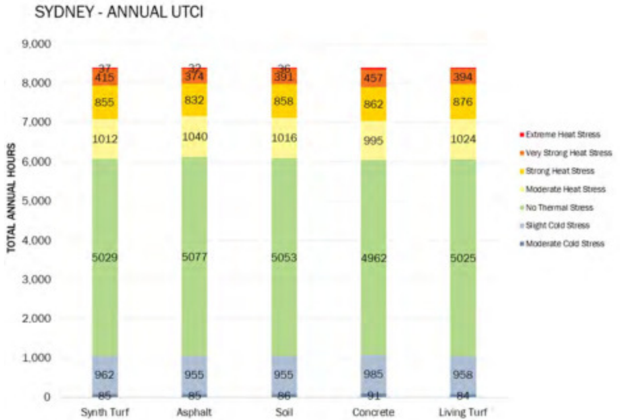
Figure 52. Sydney Annual UTCI, grouped by thermal stress.
