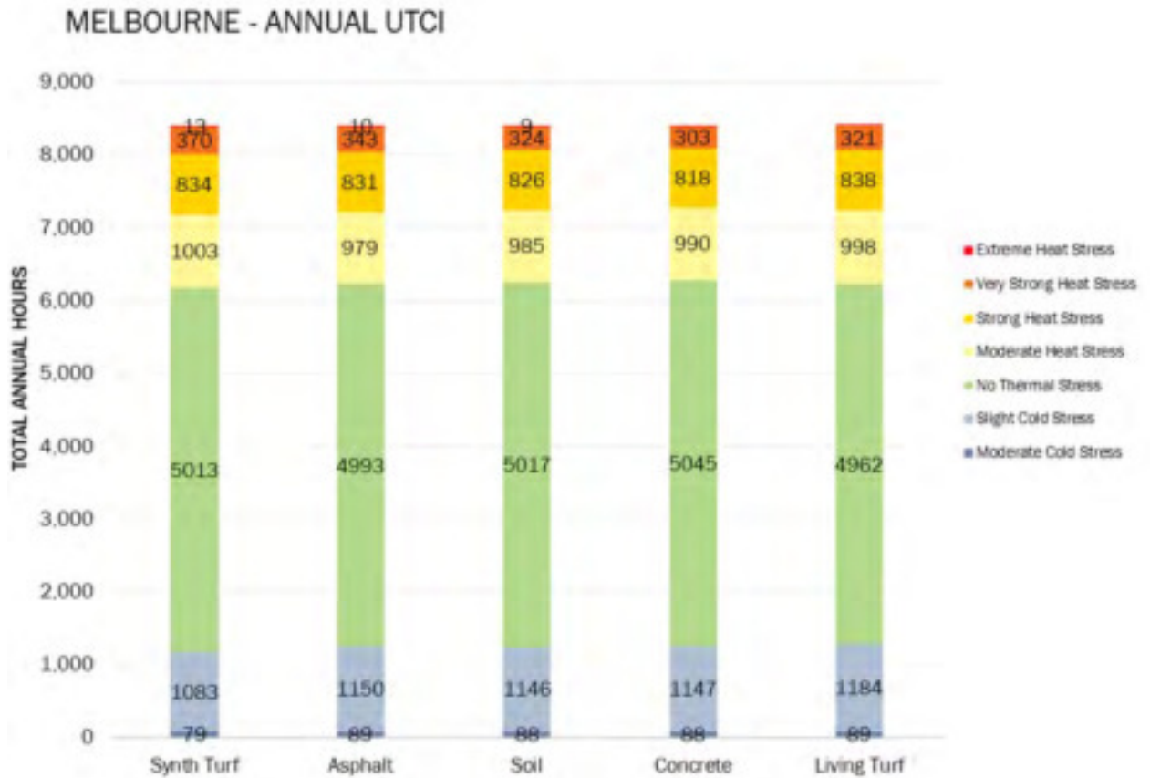
Figure 54. Melbourne Annual UTCI, grouped by thermal stress.
